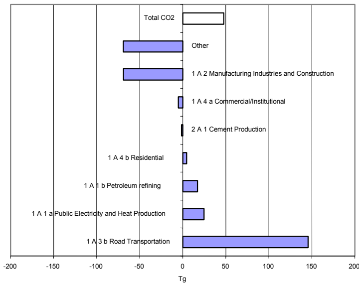
Figure 3: Absolute change of CO 2 emissions by large key source categories 1990 to 2002 in CO 2 equivalents (Tg)
