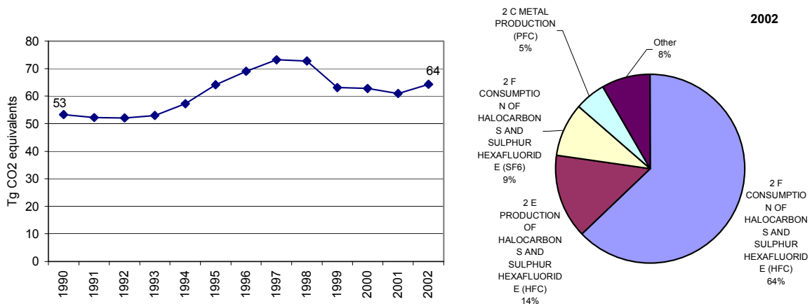
Figure 8: Fluorinated gas emissions 1990 to 2002 in CO 2 equivalents (Tg) and share of largest source categories in 2002
