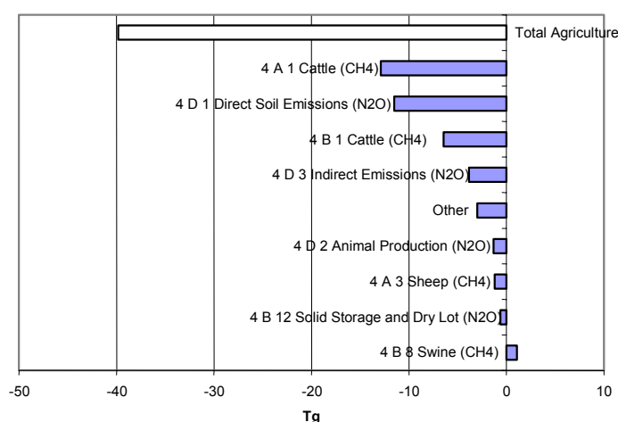
Figure 16: Absolute change of GHG emissions by large key source categories 1990-2002 in CO 2 equivalents (Tg) in CRF Sector 4, 'Agriculture'
