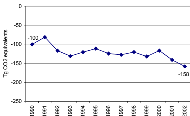
Figure 17: EC net GHG emissions (emissions minus removals) for 1990–2002 from CRF Sector 5, ‘LUCF’ in CO 2 equivalents (Tg)
