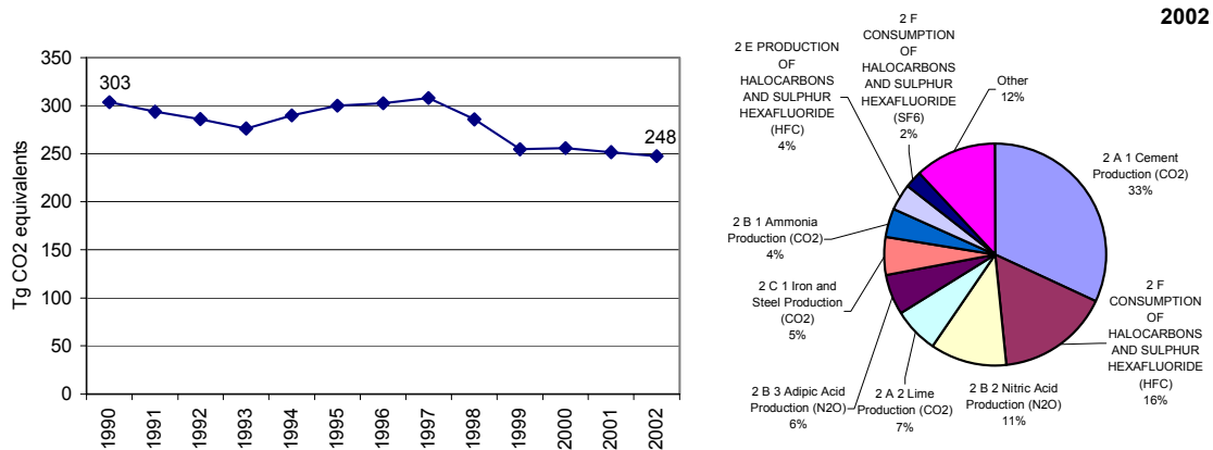
Figure 12: EC GHG emissions for 1990-2002 from CRF Sector 2, 'Industrial processes' in CO 2 equivalents (Tg) and share of largest key source categories in 2002
