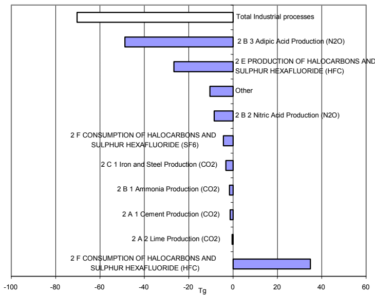
Figure 13: Absolute change of GHG emissions by large key source categories base year to 2002 in CO 2 equivalents (Tg) in CRF Sector 2, 'Industrial processes'
