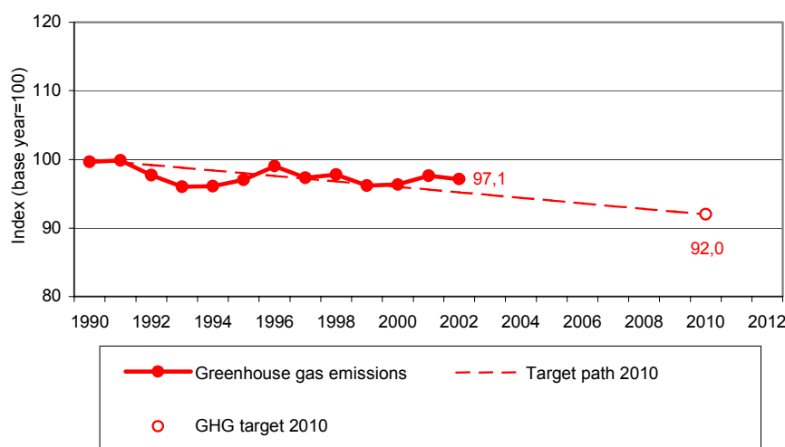
Figure 1: EC GHG emissions 1990-2002 compared with target for 2008-2012 (excl. LUCF)
