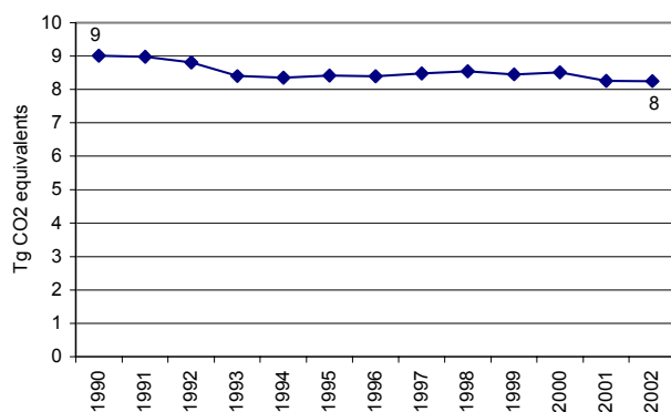
Figure 14: EC GHG emissions for 1990-2002 from CRF Sector 3, ‘Solvent and other product use’ in CO 2 equivalents (Tg) and share of largest source categories in 2002
