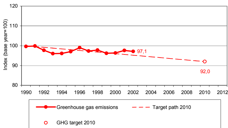
Figure ES.1: EC GHG emissions 1990-2002 compared with target for 2008-2012 (excl. LUCF)
