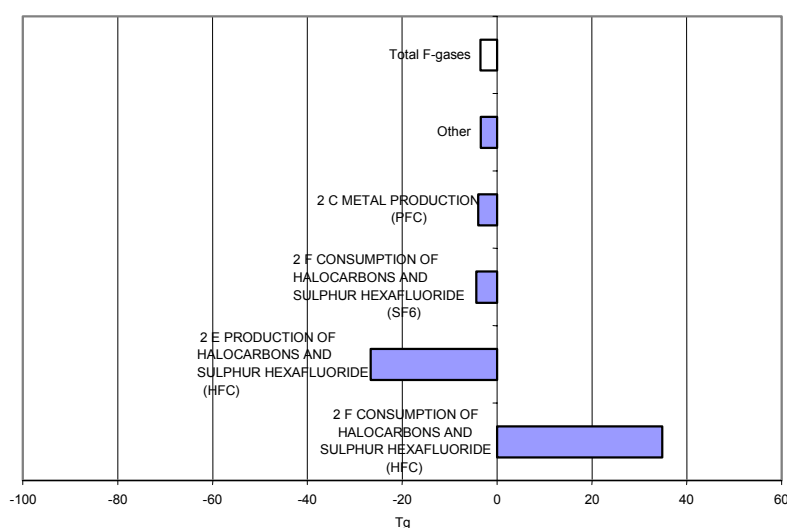
Figure 9: Absolute change of fluorinated gas emissions by large key source categories base year to 2002 in CO 2 equivalents (Tg)
