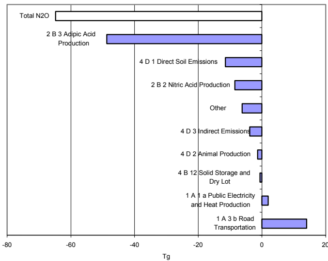
Figure 7: Absolute change of N 2 O emissions by large key source categories 1990 to 2002 in CO 2 equivalents (Tg)
