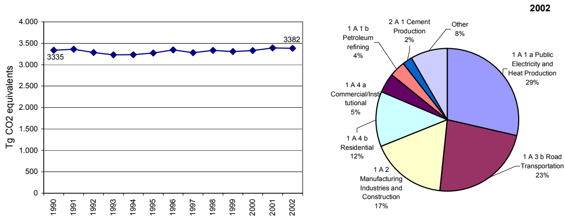
Figure 2: CO 2 emissions without LUCF 1990 to 2002 in CO 2 equivalents (Tg) and share of largest key source categories in 2002
