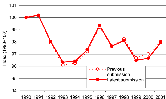
Figure 21: Comparison of EC GHG emission trends 1990-2001 (excl. LUCF) of the latest and the previous submission
