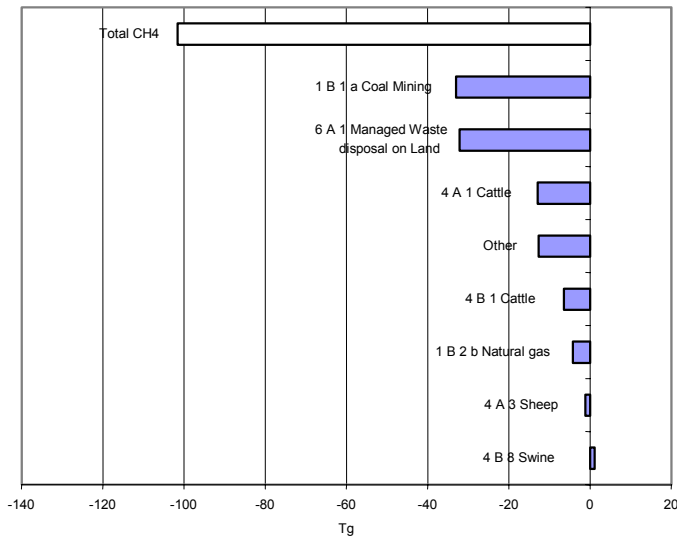
Figure 5: Absolute change of CH 4 emissions by large key source categories 1990 to 2002 in CO 2 equivalents (Tg)
