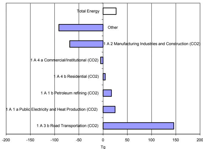
Figure 11: Absolute change of GHG emissions by large key source categories 1990-2002 in CO 2 equivalents (Tg) in CRF Sector 1, 'Energy'
