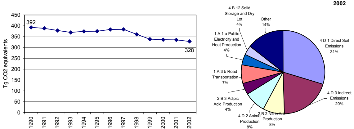
Figure 6: N 2 O emissions 1990 to 2002 in CO 2 equivalents (Tg) and share of largest source categories in 2002
