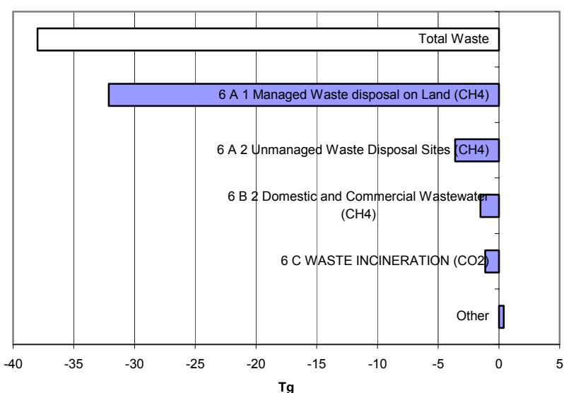
Figure 19: Absolute change of GHG emissions by large key source categories 1990-2002 in CO 2 equivalents (Tg) in CRF Sector 6, 'Waste'
