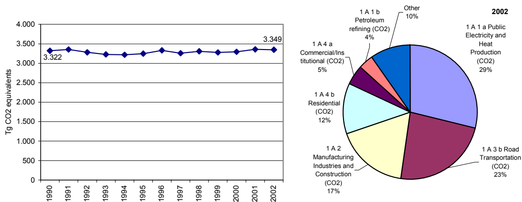
Figure 10: EC GHG emissions for 1990-2002 from CRF Sector 1, 'Energy' in CO 2 equivalents (Tg) and share of largest key source categories in 2002
