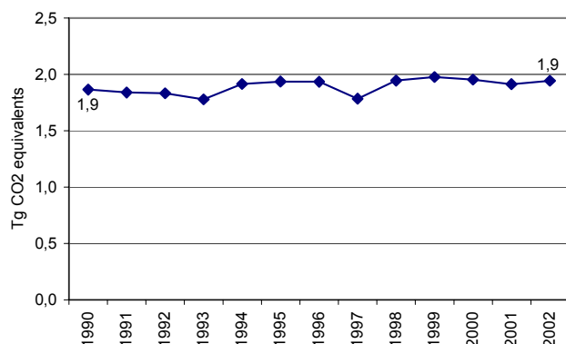
Figure 20: EC GHG emissions 1990-2002 from CRF sector 7 ‘Other’ in CO 2 equivalents (Tg)
