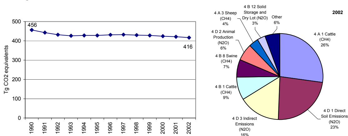
Figure 15: EC GHG emissions for 1990-2002 from CRF Sector 4, ‘Agriculture’ in CO 2 equivalents (Tg) and share of largest key source categories in 2002
