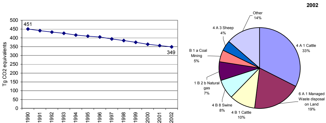
Figure 4: CH 4 emissions 1990 to 2002 in CO 2 equivalents (Tg) and share of largest source categories in 2002
